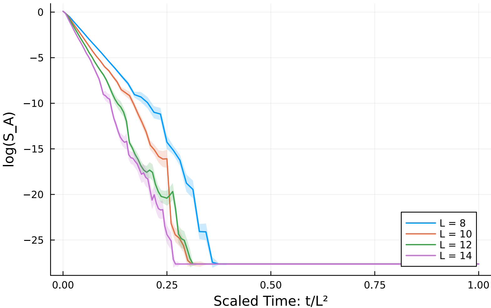
Scaled Log Entropy Evolution ( p = 0.716667 )
